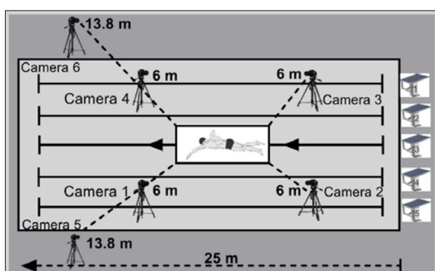
Figure 1 Positioning of the cameras for 3D analysis and the calibrated space.
